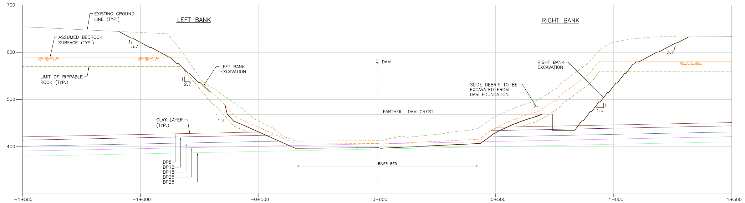
SECTION ALONG DAM AXIS C2
