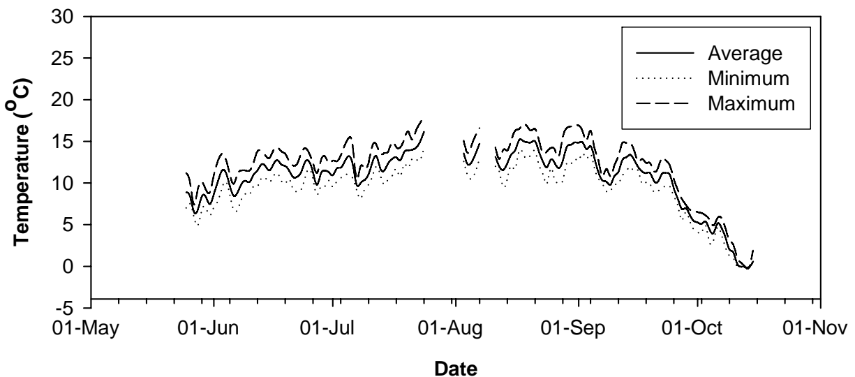
Figure 3.4 Daily water temperatures of the upper Halfway River, 2009 Peace River tributaries water temperature monitoring study.
