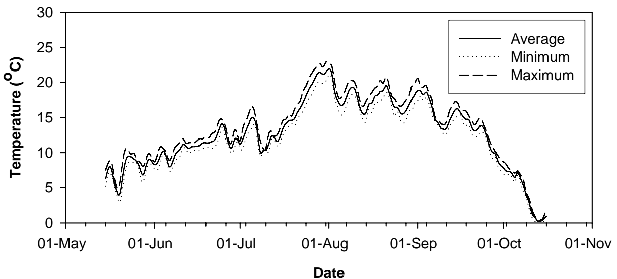
Figure 3.8 Daily water temperatures of the Pine River, 2009 Peace River tributaries water temperature monitoring study.
