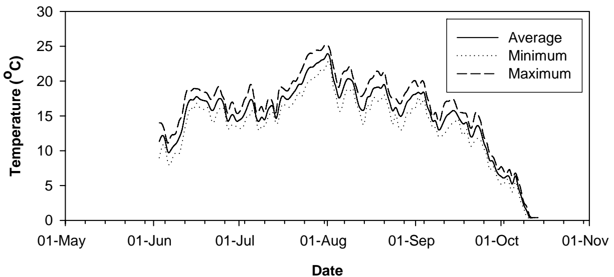
Figure 3.6 Daily water temperatures of the upper Moberly River, 2009 Peace River tributaries water temperature monitoring study.
