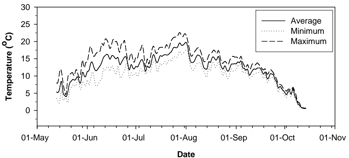
Figure 3.2 Daily water temperatures of Lynx Creek, 2009 Peace River tributaries water temperature monitoring study.
