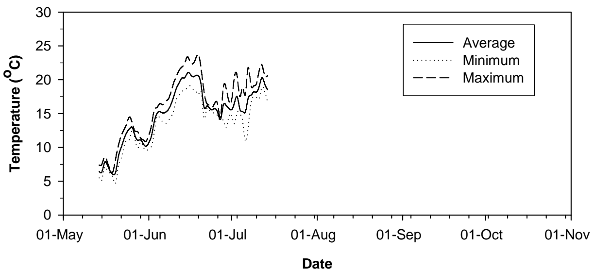
Figure 3.9 Daily water temperatures of the Beaton River, 2009 Peace River tributaries water temperature monitoring study.
