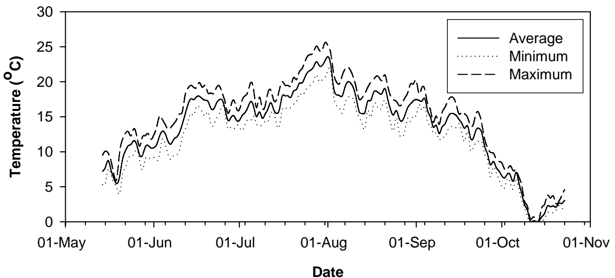
Figure 3.7 Daily water temperatures of the lower Moberly River, 2009 Peace River tributaries water temperature monitoring study.
